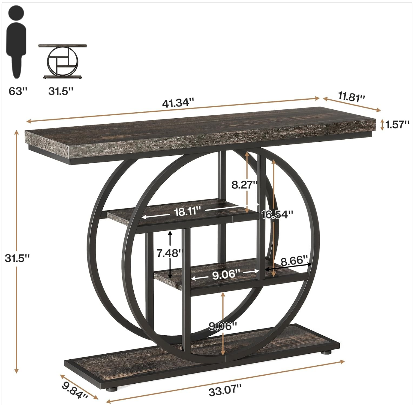
Figure 3.1: Detailed dimensions of the console table, including shelf spacing.
