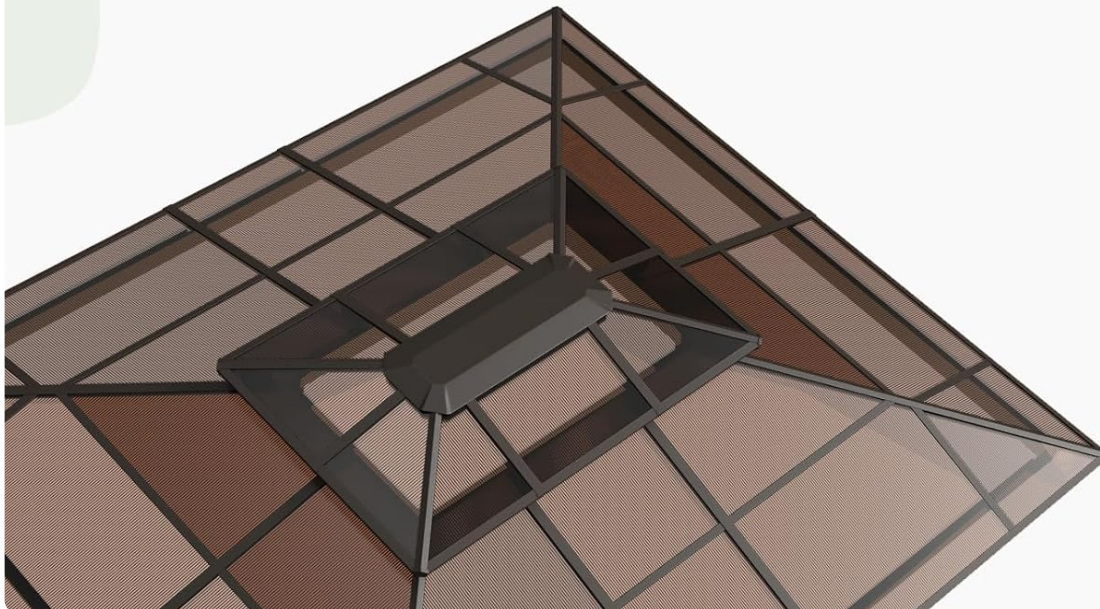
Figure 3.1: The double roof design ensures air ventilation and features a water gutter system for smooth drainage, preventing water accumulation.
