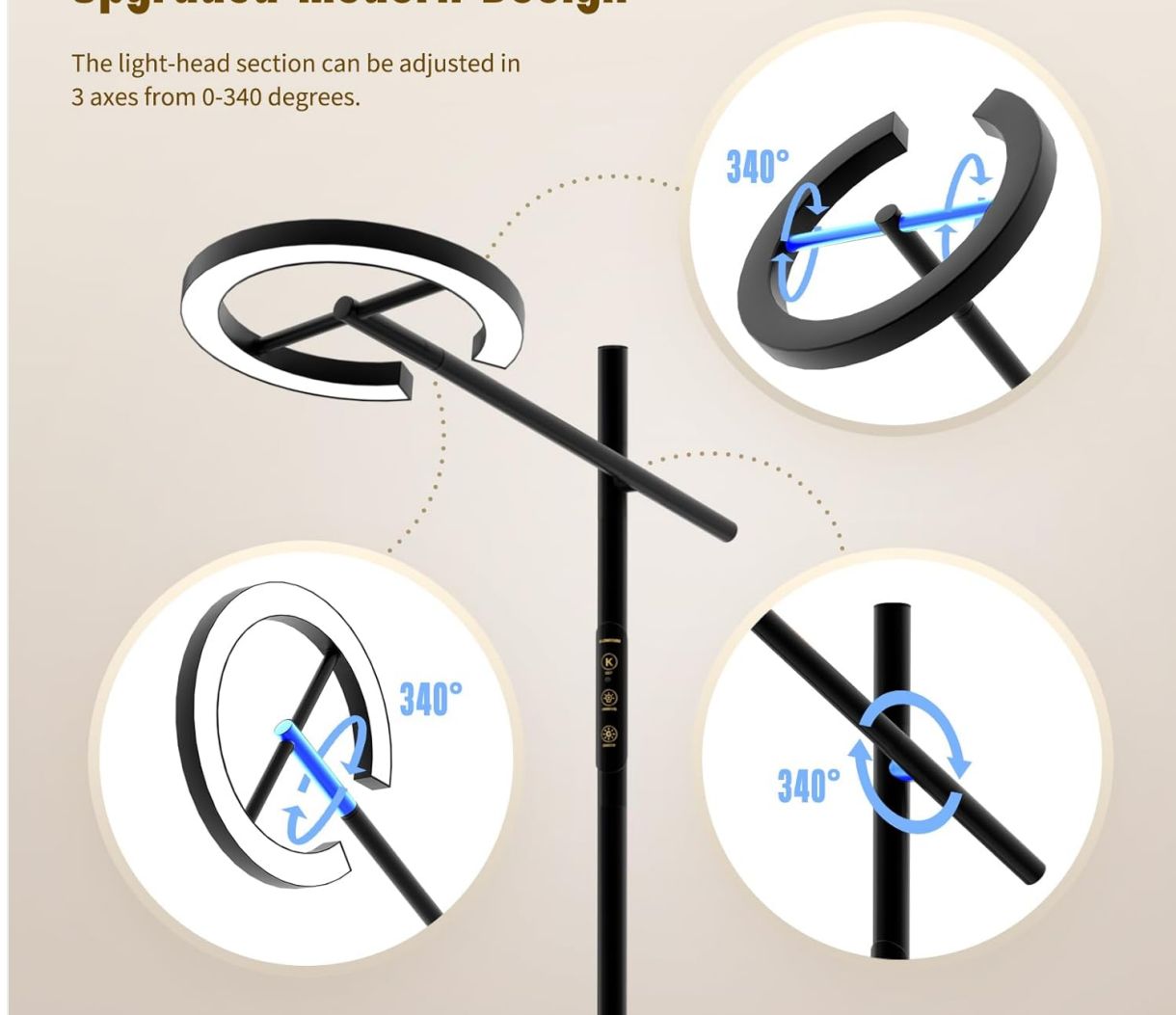
Figure 5.3: Lamp head rotation for directional lighting.
