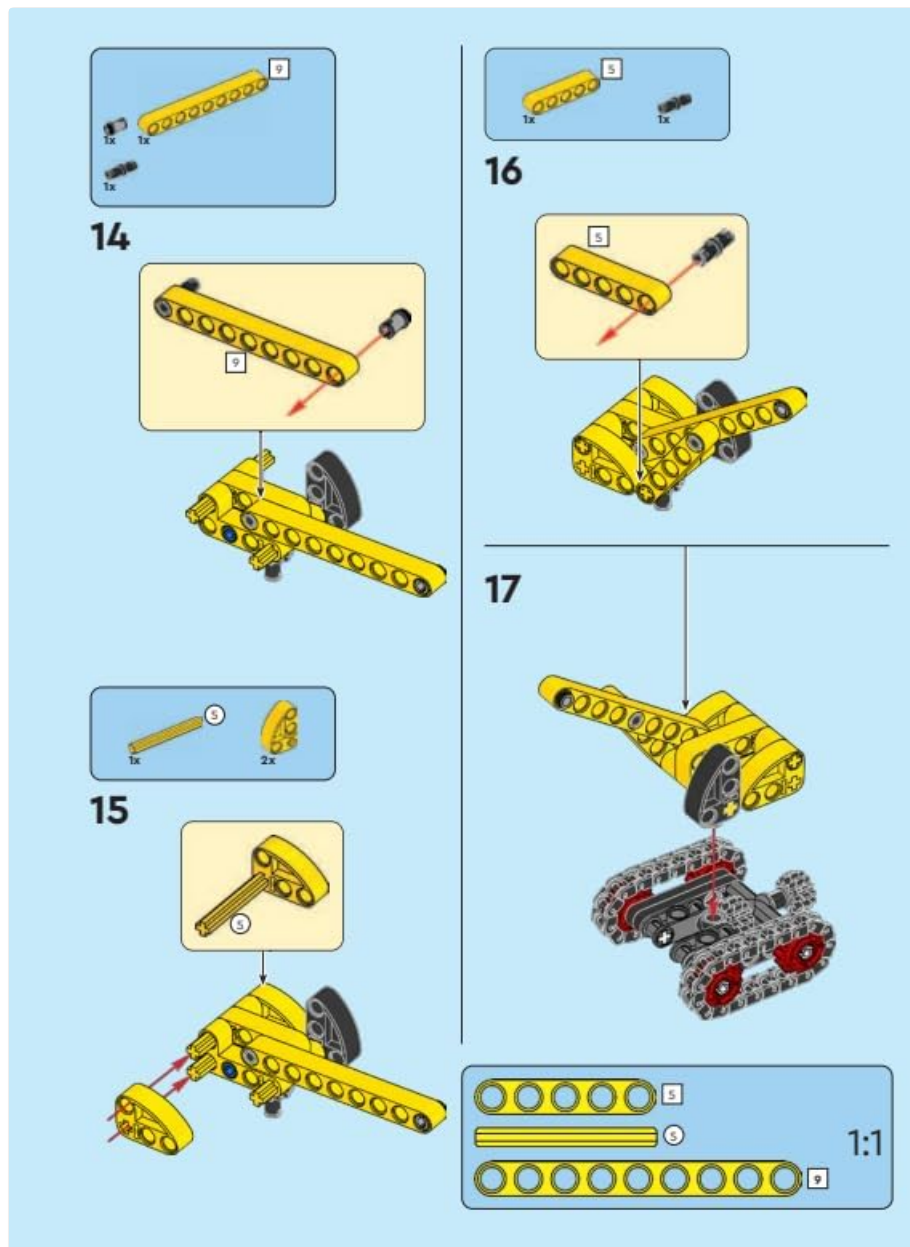
Figure 7: Assembly steps 16 and 17. This section shows how to connect the completed crane arm assembly to the tracked chassis.
