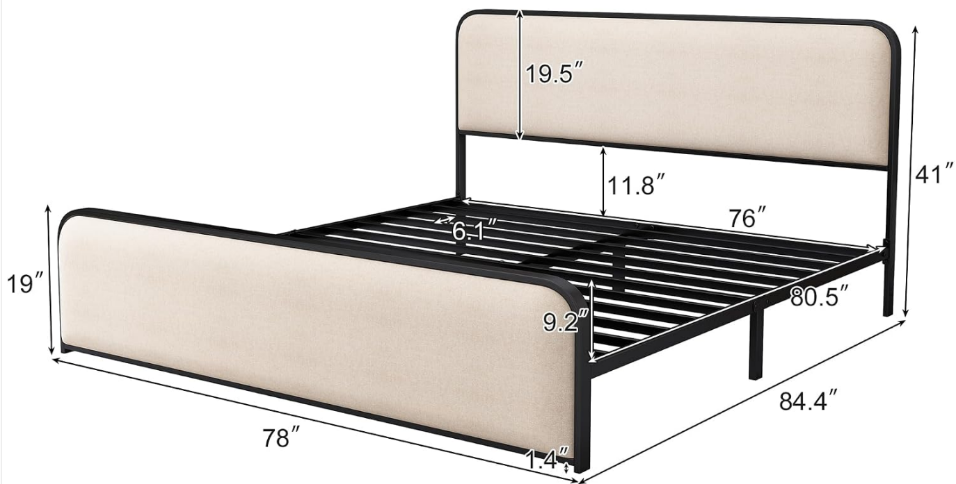
Image: A detailed diagram showing the dimensions of the King size bed frame in inches, including overall length, width, height, headboard height, and underbed clearance.
