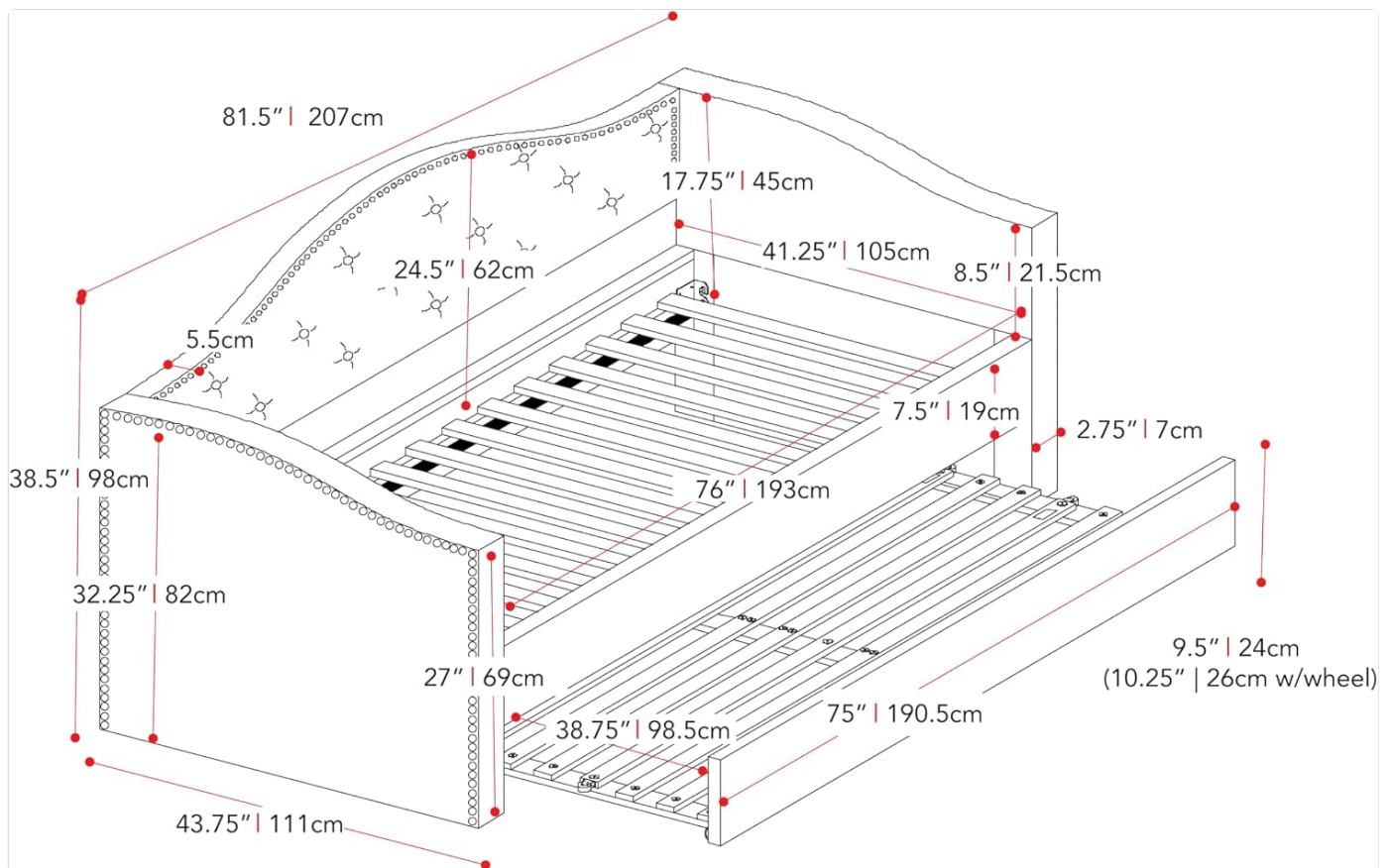
Image: All components of the CorLiving Everly Day Bed with Trundle laid out for assembly.
