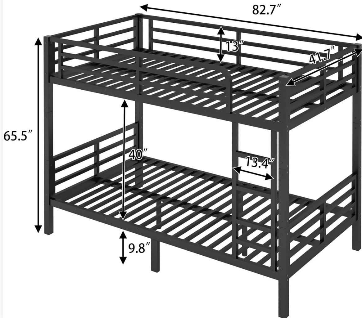
Image: Diagram illustrating the dimensions of the Bellemave Twin XL Over Twin XL Bunk Bed.
