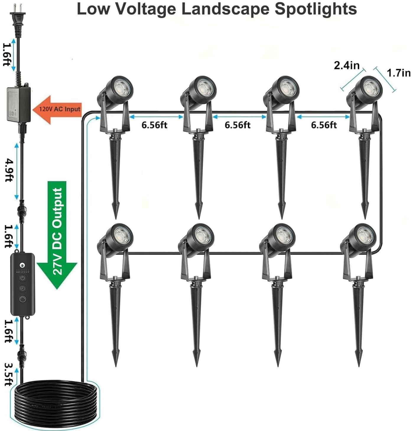
Figure 3.2: System Connection and Dimensions
