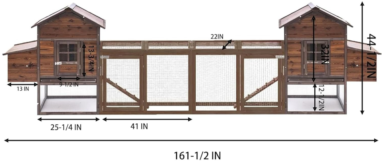
Image 8.1: Detailed dimensional drawing of the chicken coop, indicating overall length, width, and height, as well as specific measurements for different sections.
