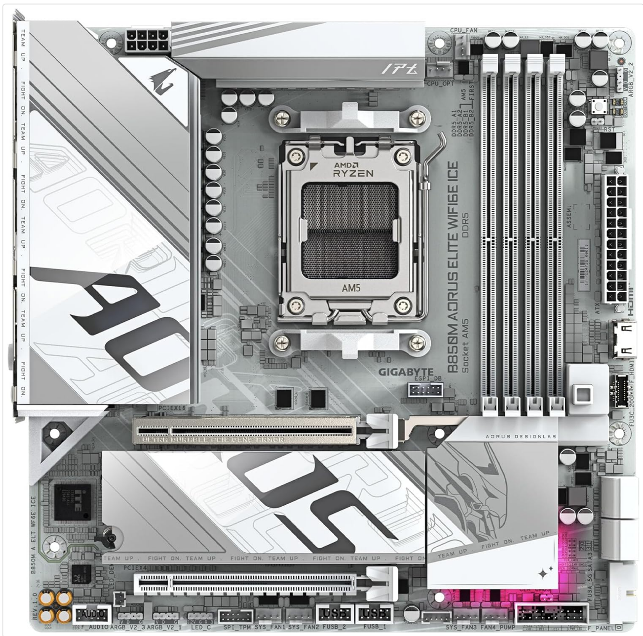
An overhead view of the motherboard, detailing the CPU socket, PCIe slots, and M.2 slots with their thermal guards.
