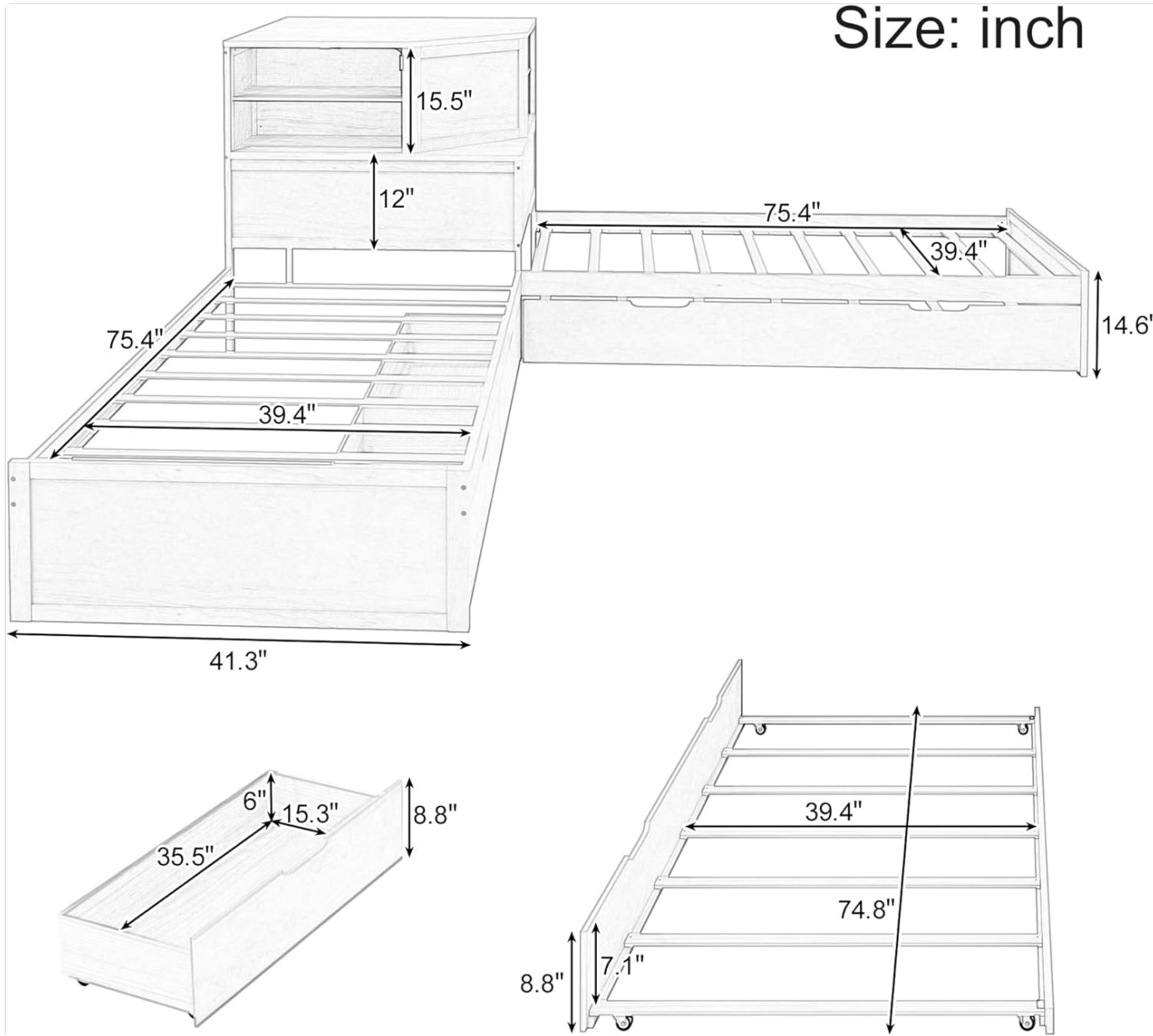
Image: A detailed diagram showing the dimensions of the L-shaped bed, including the main bed frames, the trundle, and the storage drawers, with measurements in inches.
