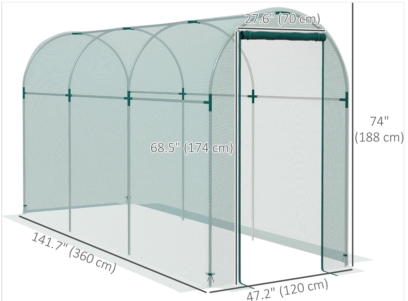
Image: A technical diagram illustrating the overall dimensions and door size of the Outsunny Crop Cage.
