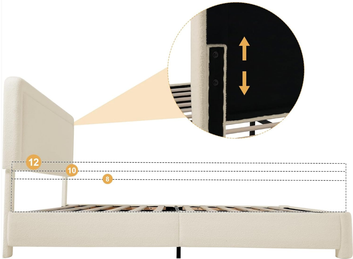
Image 3.2: Detail of the sturdy metal frame and the convenient Velcro slat system for noise-free support.
