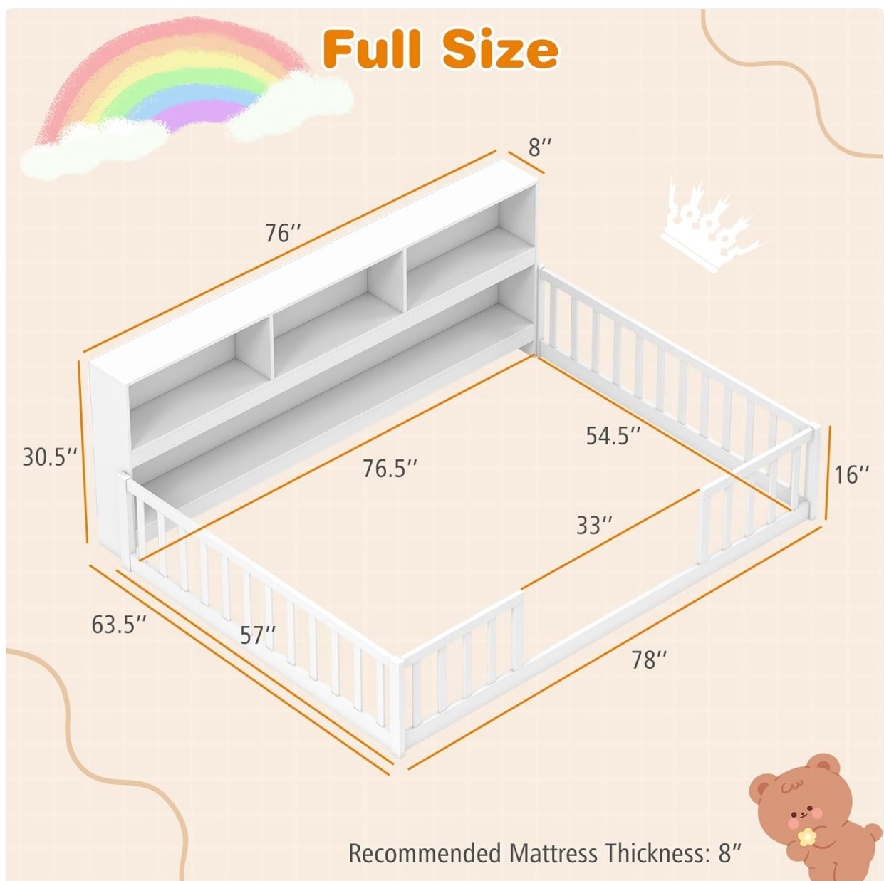
Figure 2: Product dimensions for the Full Size Montessori Floor Bed.
