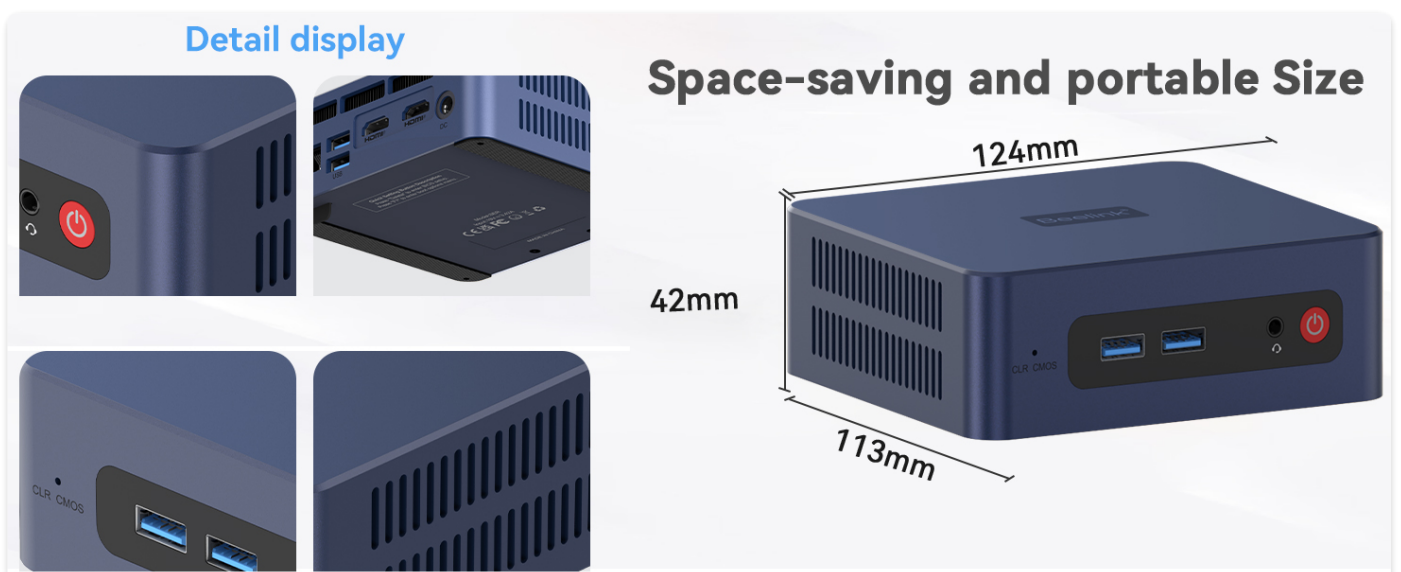
The compact design of the Beelink SER3 Mini PC, highlighting its small footprint and detailed features.
