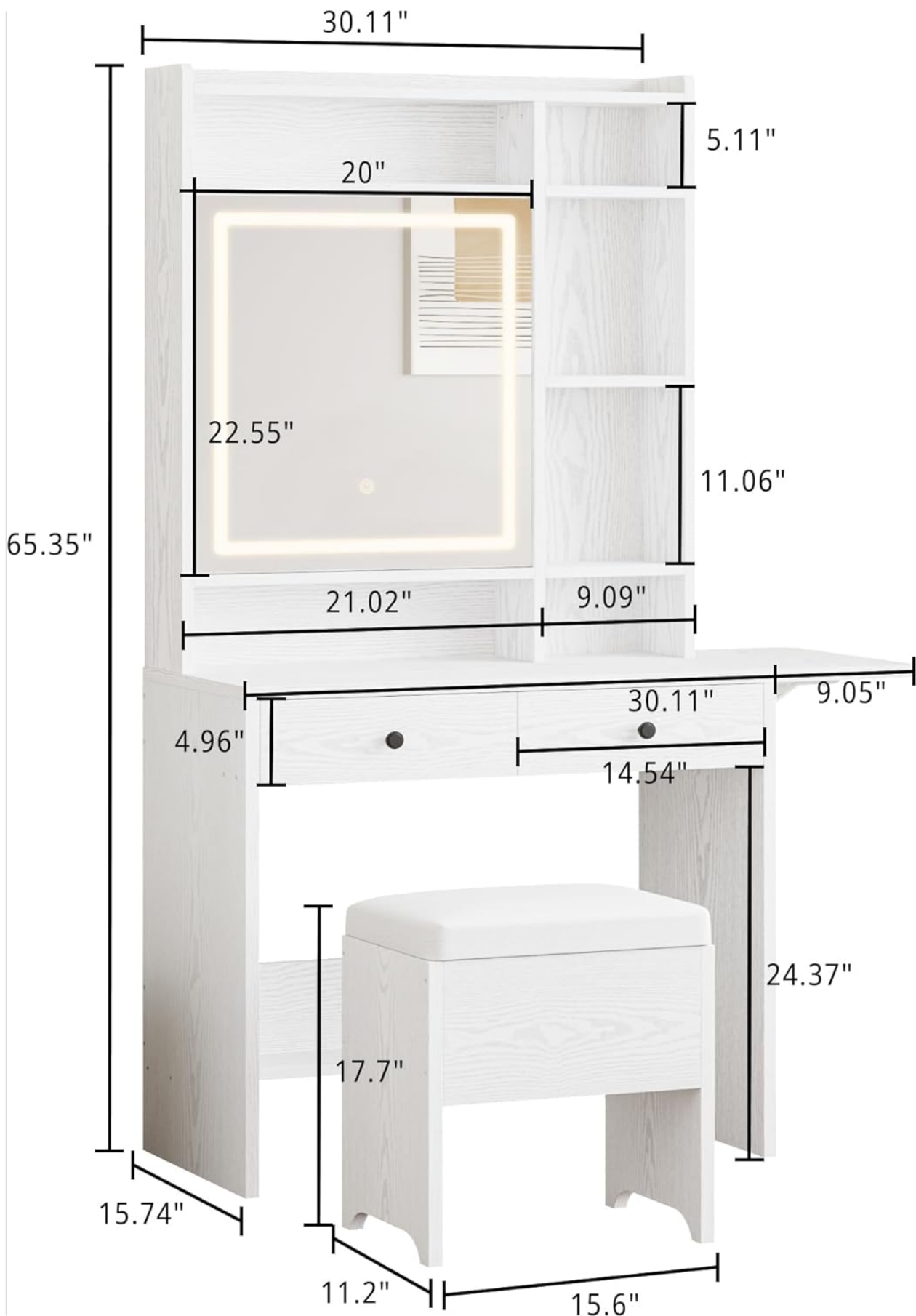
Image Description: A technical drawing displaying the complete dimensions of the vanity desk, including measurements for the mirror, shelves, drawers, and overall structure.
