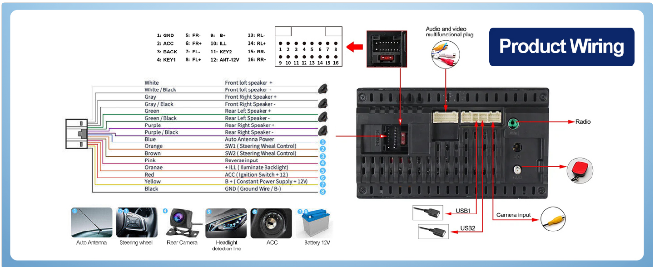
Image: Product Wiring Diagram.
