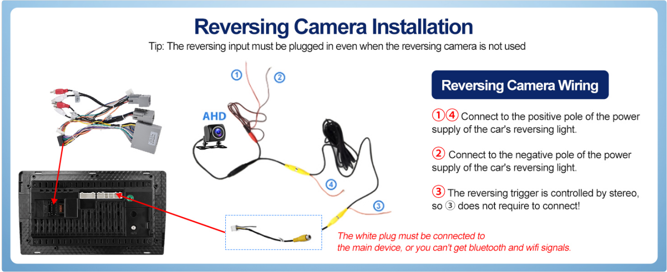
Image: Reversing Camera Wiring Diagram.
