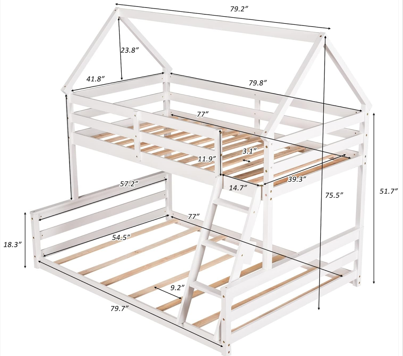
Image: Detailed dimensions of the Bellemave Twin Over Full House Bunk Bed, showing length, width, and height measurements for both bunks and the overall structure.
