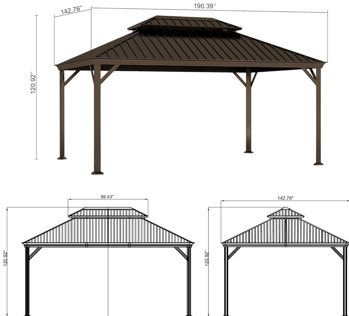
Image 7.1: Dimensional overview of the Domi Hardtop Gazebo.
