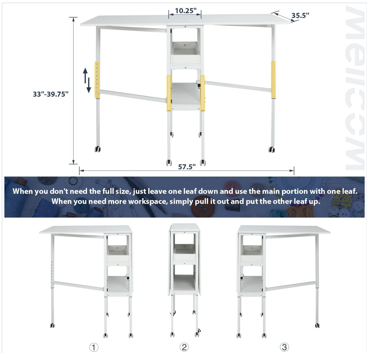
Image 5.2: A diagram detailing the table's dimensions and demonstrating its versatile folding capabilities, from fully extended to a compact, folded state.
