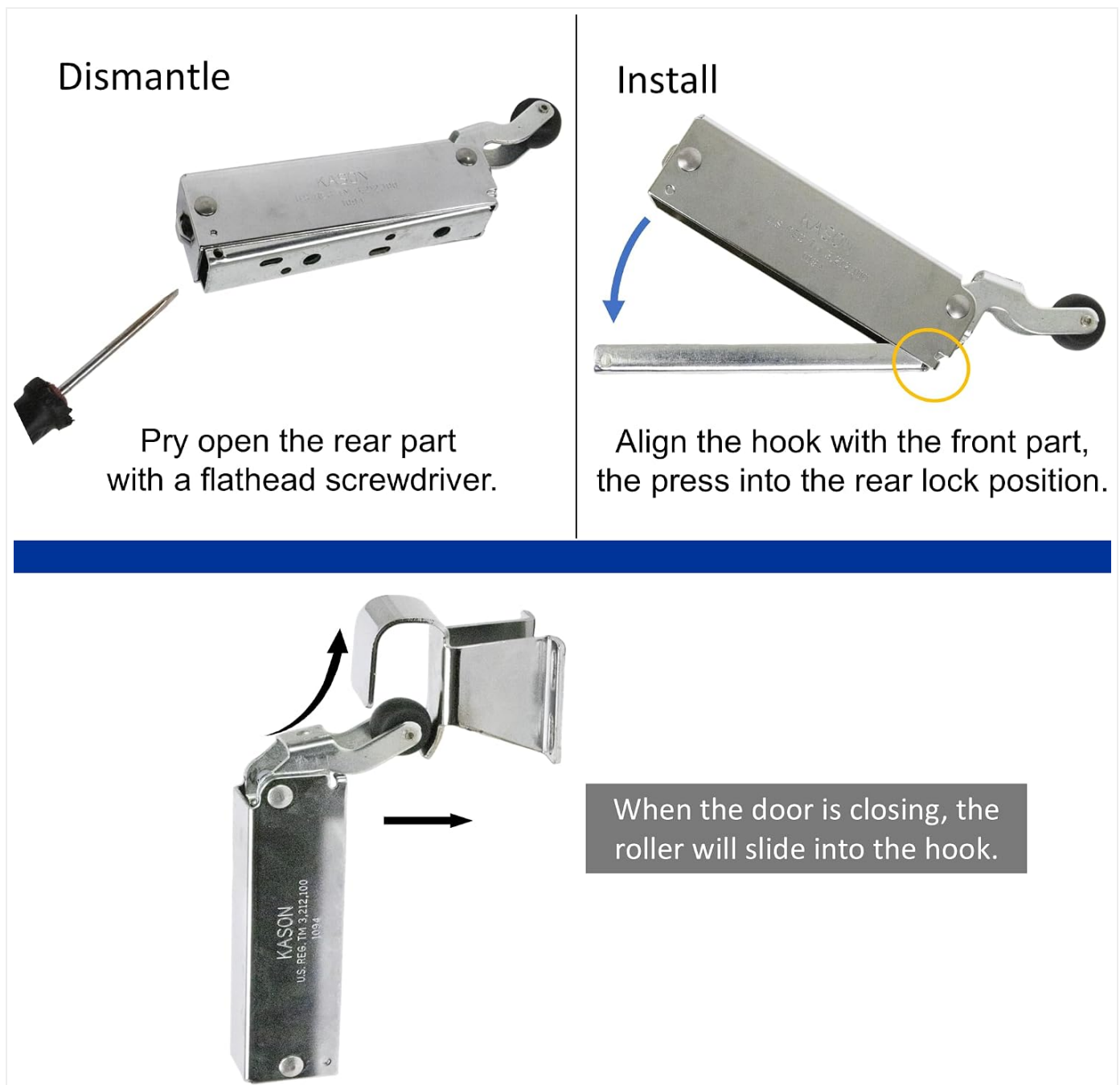
Image 4.2: Illustration of the installation process, showing how to dismantle (pry open rear part with flathead screwdriver) and install (align hook with front part, press into rear lock position) the door closer components. It also shows how the roller slides into the hook during door closure.
