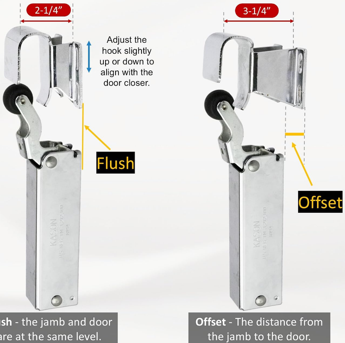
Image 4.1: Visual guide for understanding and measuring door offset. This helps determine if your door requires a flush or offset hook configuration.
