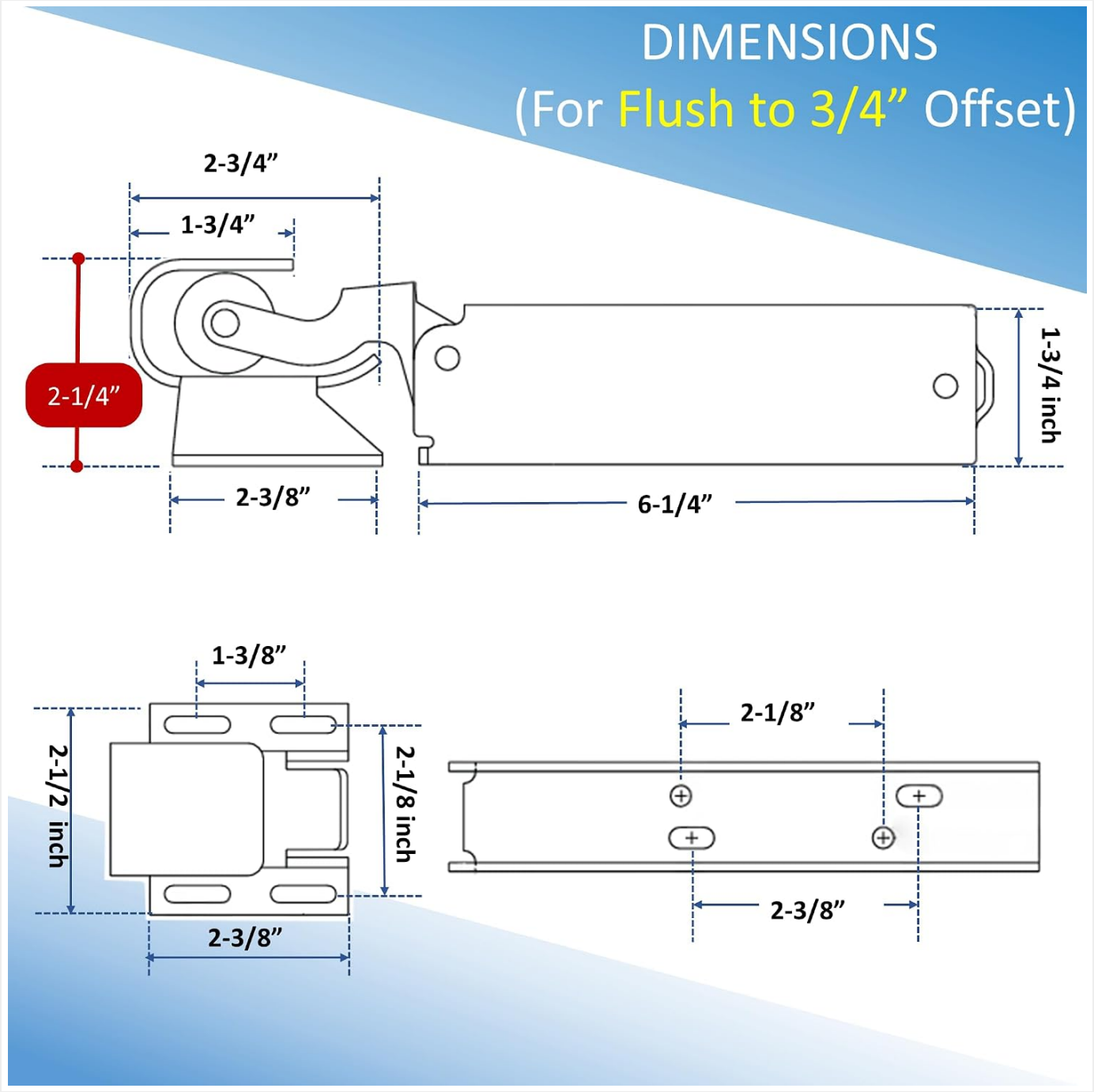
Image 8.1: Detailed dimensions of the Kason 1094 Hydraulic Door Closer and its hook for flush to 3/4 inch offset applications.
