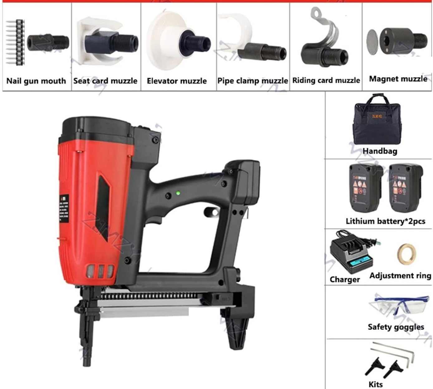
Figure 3.2: Multifunctional Gas Nail Gun with included accessories. This image illustrates different muzzle attachments (nail gun mouth, seat card muzzle, elevator muzzle, pipe clamp muzzle, riding card muzzle, magnet muzzle) and additional items such as a handbag, two lithium batteries, a charger, an adjustment ring, safety goggles, and kits (wrenches).
