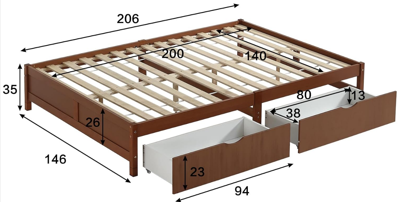
Image: A technical diagram illustrating the overall dimensions of the Moimhear bed frame (206x146x35 cm) and the internal dimensions of the storage drawers (94x38x23 cm).
