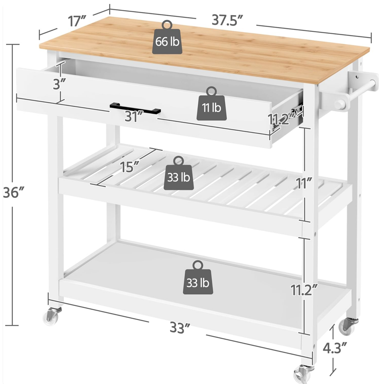
Image: A detailed diagram illustrating the dimensions of the kitchen island cart (37.5" W x 17" D x 36" H) and the maximum weight capacities for its components: 66 lbs for the countertop, 11 lbs for the drawer, and 33 lbs for each shelf.
