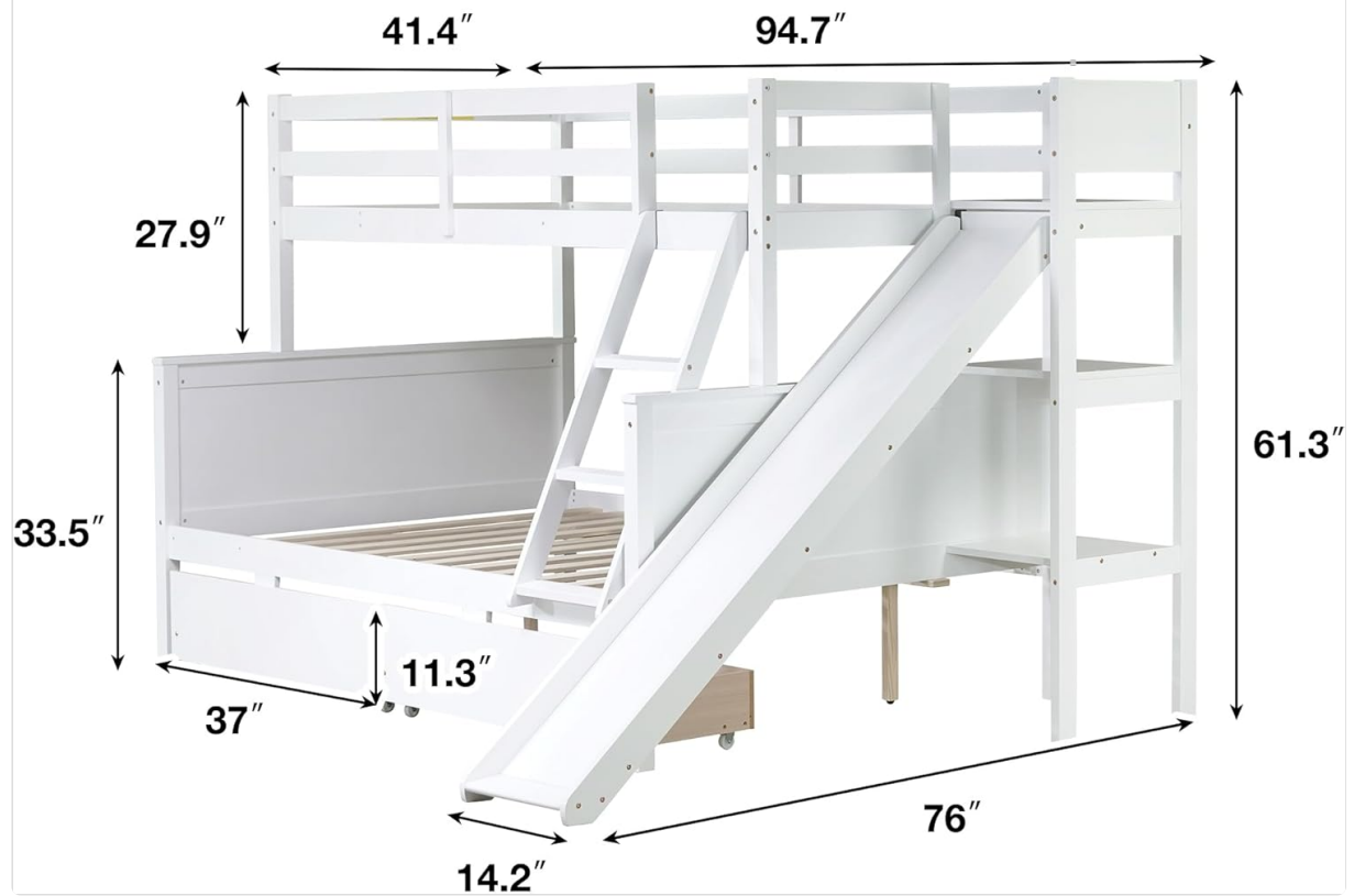
Image: Dimensional drawing of the bunk bed, indicating overall length, width, and height measurements.
