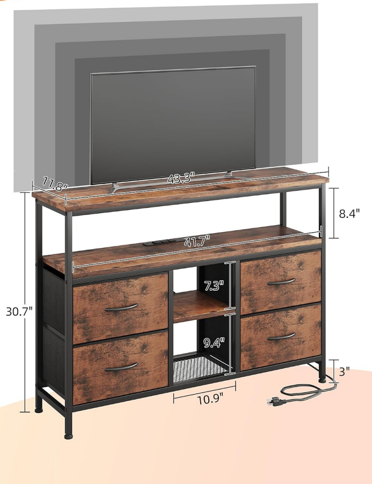
Image 4.1: Product dimensions and component breakdown.
