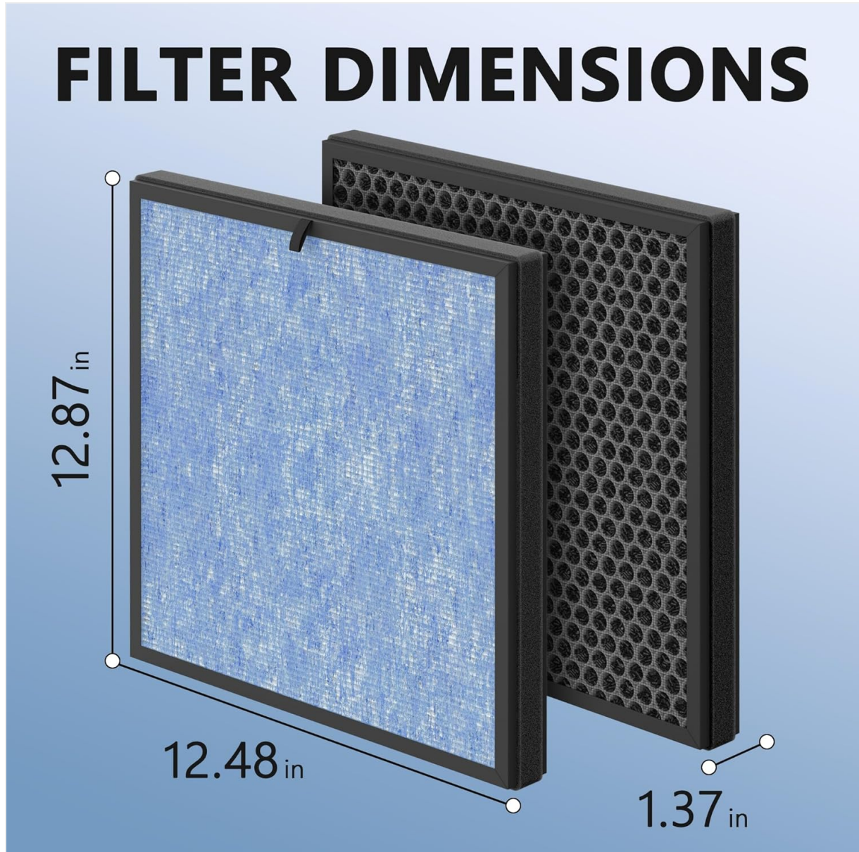
Image: Detailed illustration of the Harebery KJ01 filter dimensions, including height, width, and depth.
