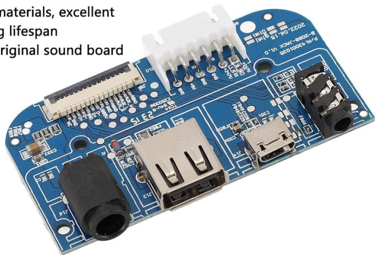
Image 1: Top view of the VBESTLIFE USB Charging Port Board, showing USB-A, Micro USB, and AC2.5 jack ports.
