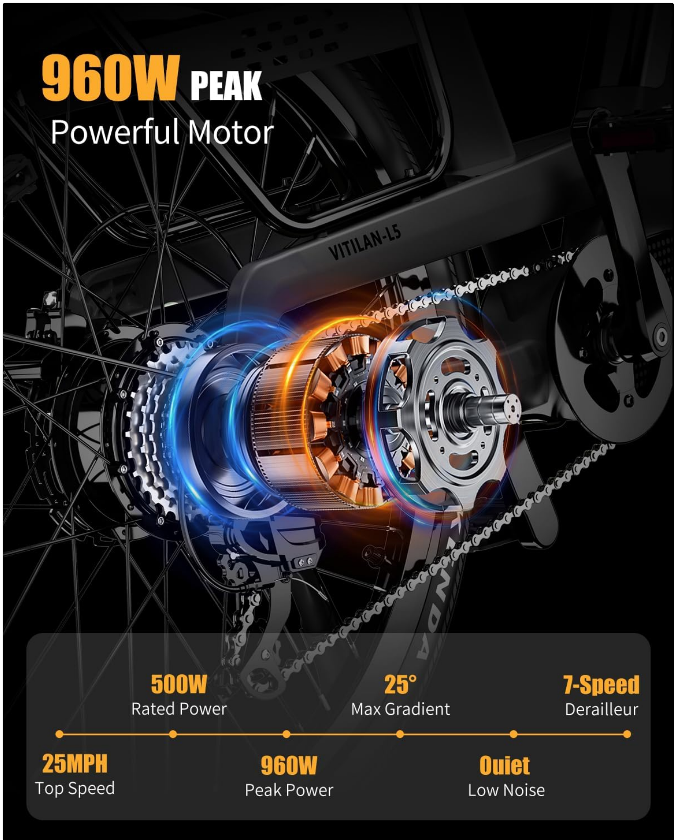
Figure 2.2: Details of the powerful 500W rated (960W peak) motor, highlighting its top speed, max gradient, and 7-speed derailleur integration.
