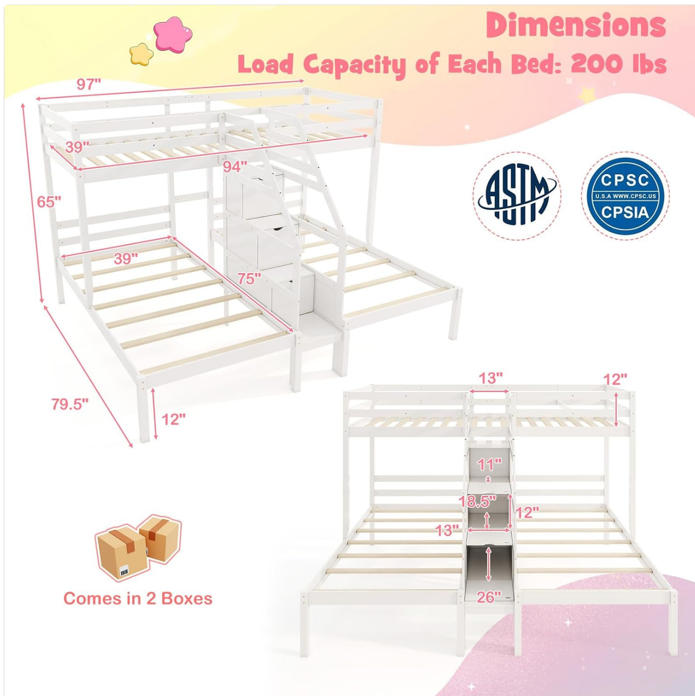
Image: Detailed dimensions of the GIANTEX Triple Bunk Bed, including length, width, height, and load capacity per bed.
