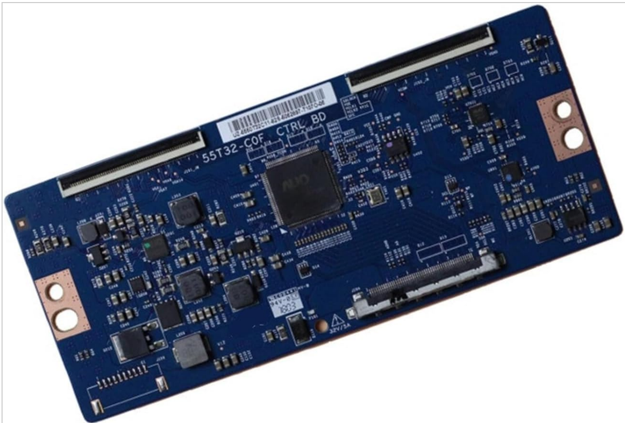
Figure 3.2: Angled view of the T-Con Board, highlighting various connectors and electronic components.
