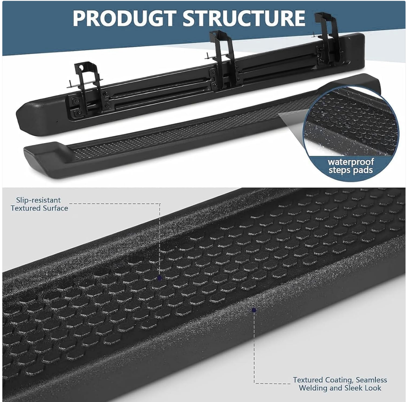
Figure 4: Product Structure. This image provides an overhead view of the running boards, showing the integrated mounting points for the brackets and a close-up of the waterproof, slip-resistant step pads.
