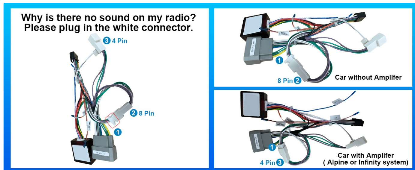
Figure 5.1: Troubleshooting for no sound issue, focusing on white connector.
