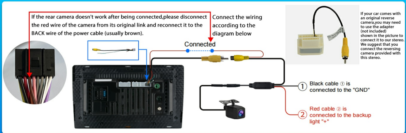
Figure 5.2: Rearview camera wiring diagram for troubleshooting.
