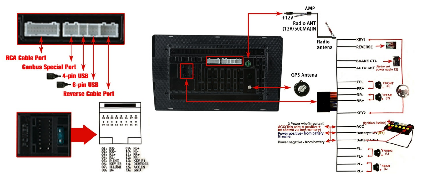
Figure 2.3: Wiring diagram for connecting the car radio.
