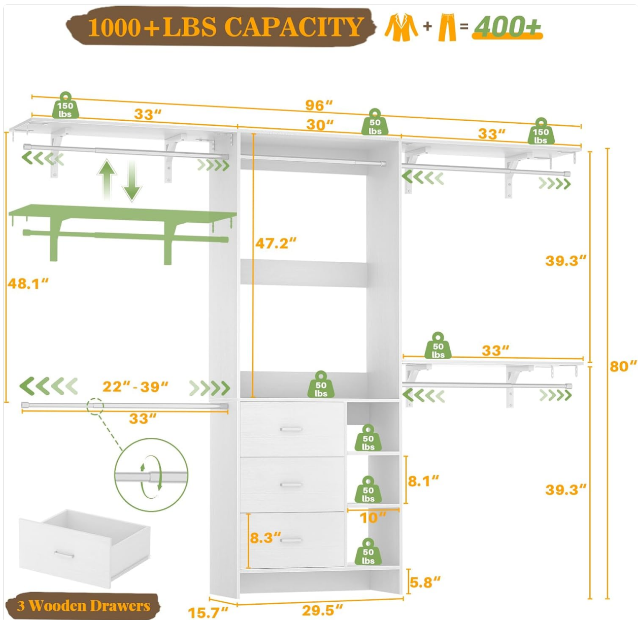
Figure 2: Flexible installation methods for adapting the closet system to various widths.
