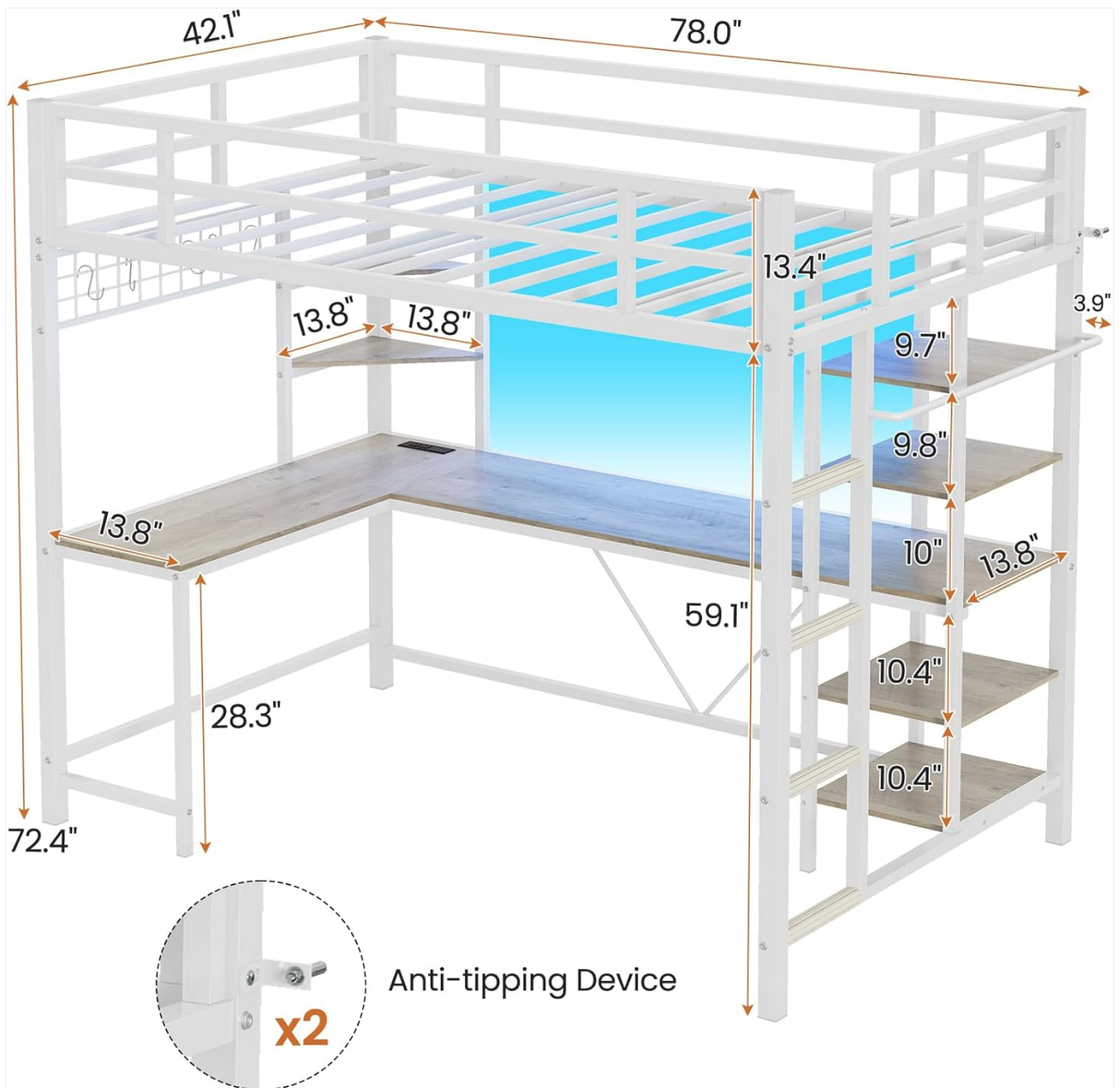
Image 8.1: Detailed dimensions of the MSmask Twin Size Loft Bed.
