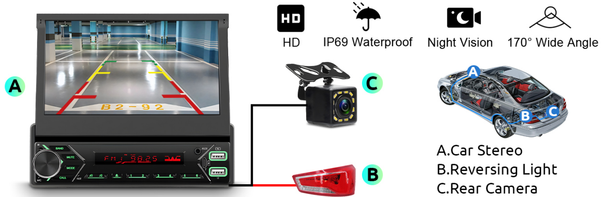
Image: Diagram illustrating the connection of the AHD backup camera to the car stereo and reversing light.
