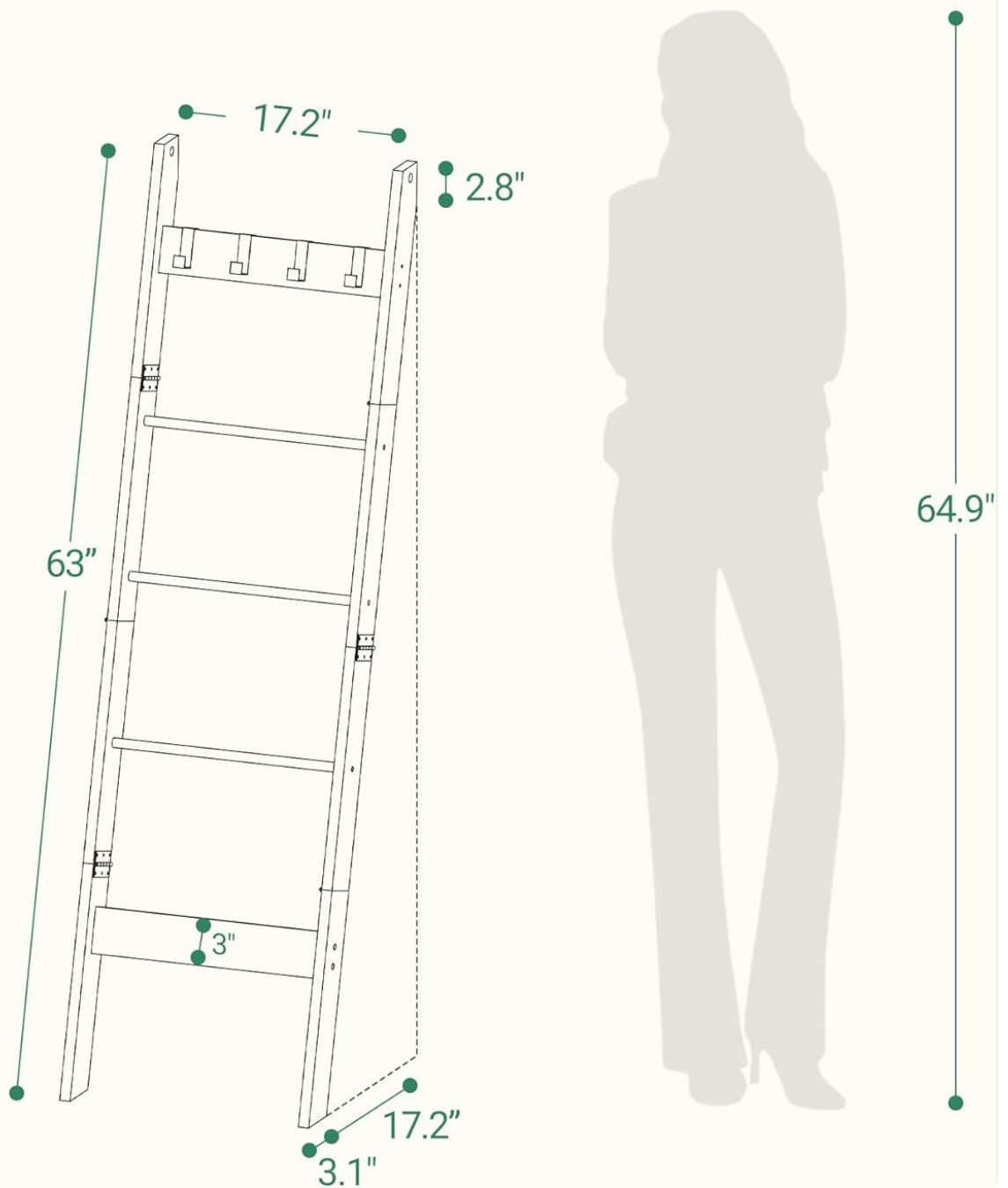
Figure 4.2: Product dimensions for planning placement.
