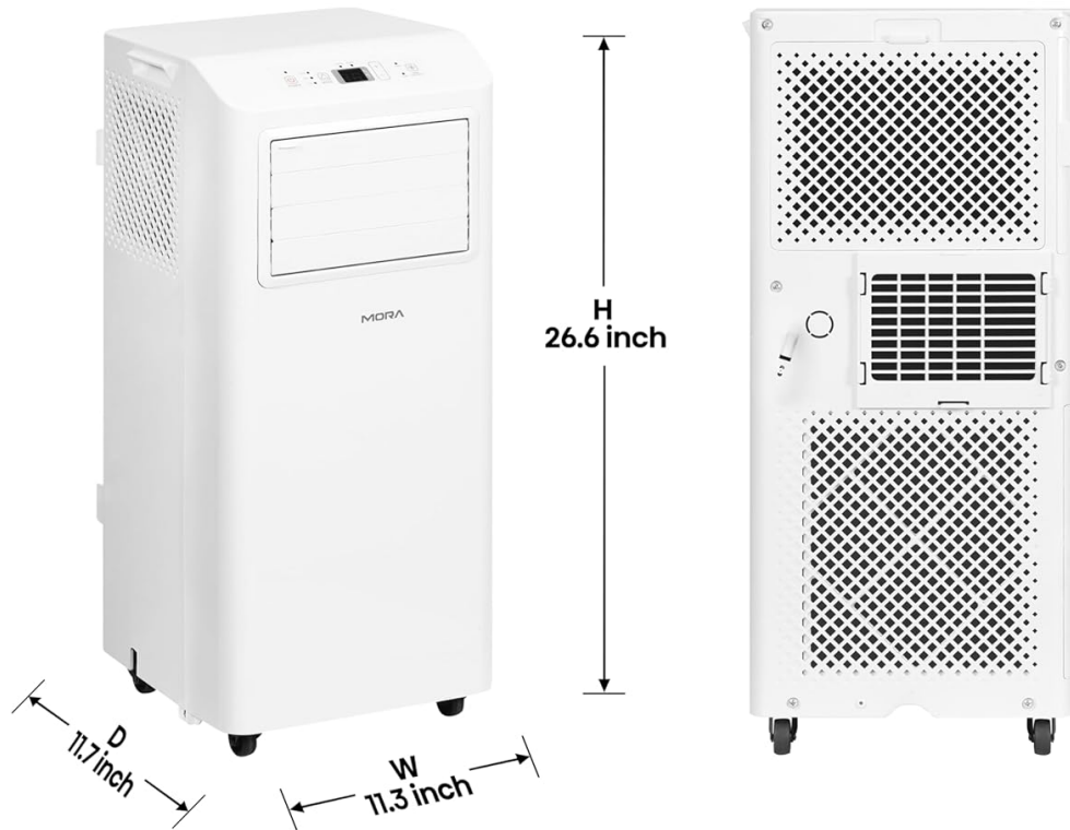
Figure 3.2: Front View
