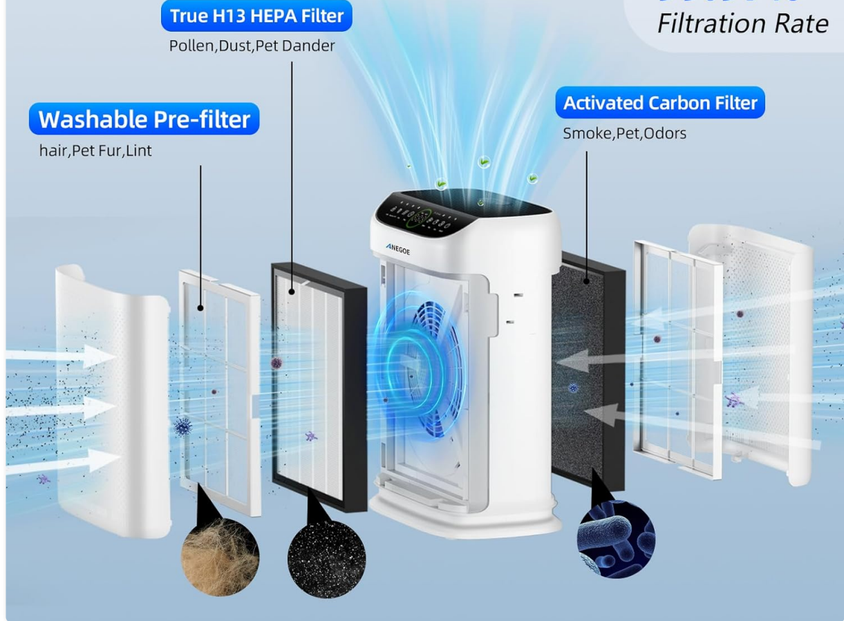
Image: Exploded view illustrating the 3-stage filtration system of the AnEgoe ZX001 air purifier.
