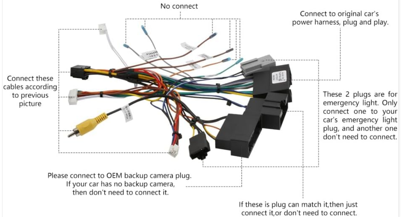
Figure 6: Visual guide on connecting various plugs during installation.
