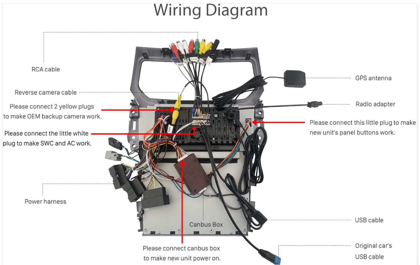
Figure 5: Detailed wiring diagram showing connections for the SEICANE H7723.
