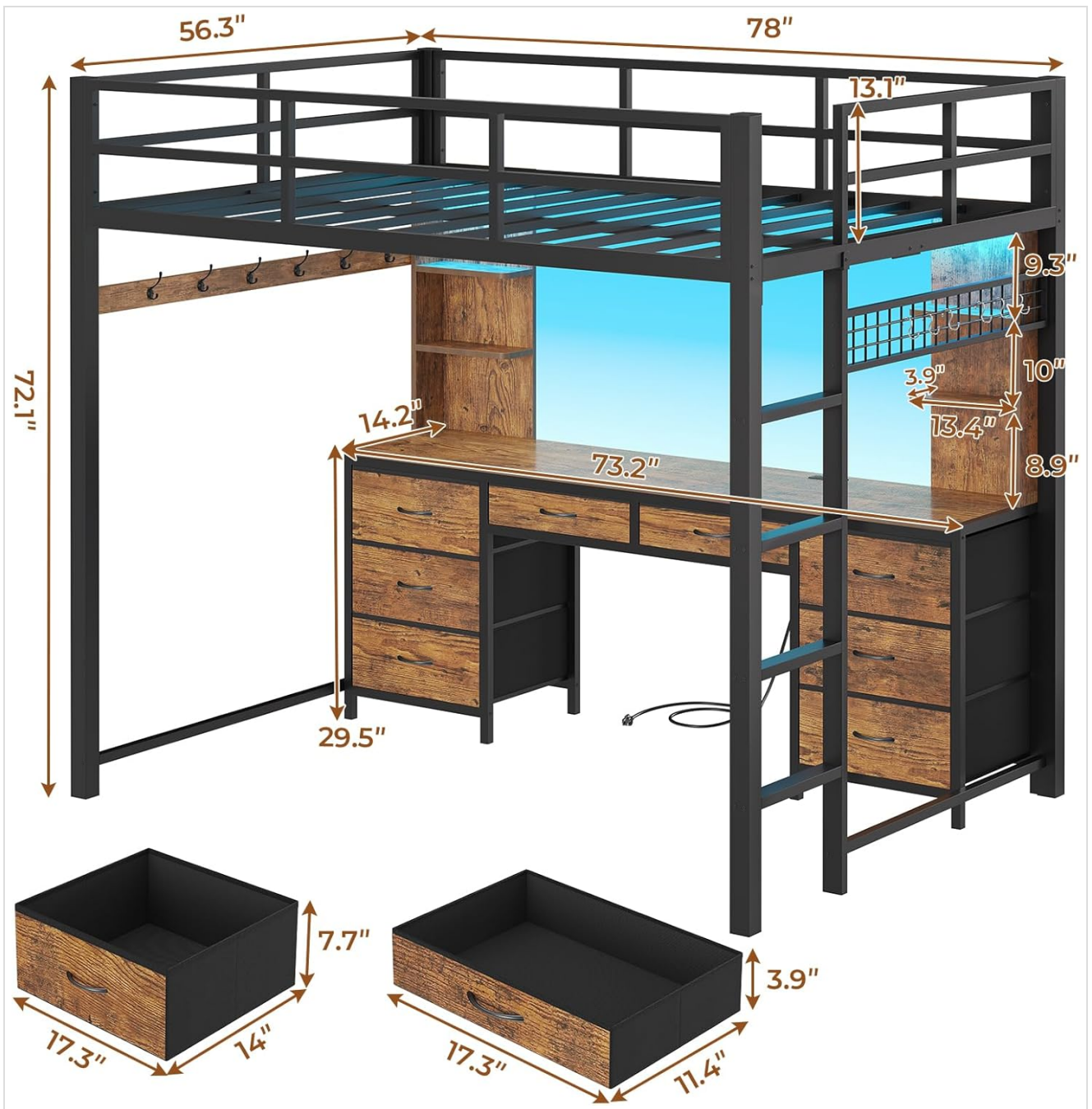
Detailed dimensions of the loft bed and its components, including the desk and drawers, aiding in assembly planning.
