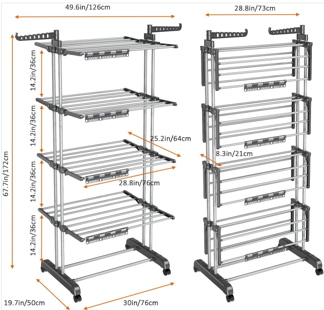
Image: A diagram illustrating the full dimensions of the drying rack when extended and folded, including height, width, and depth measurements.
