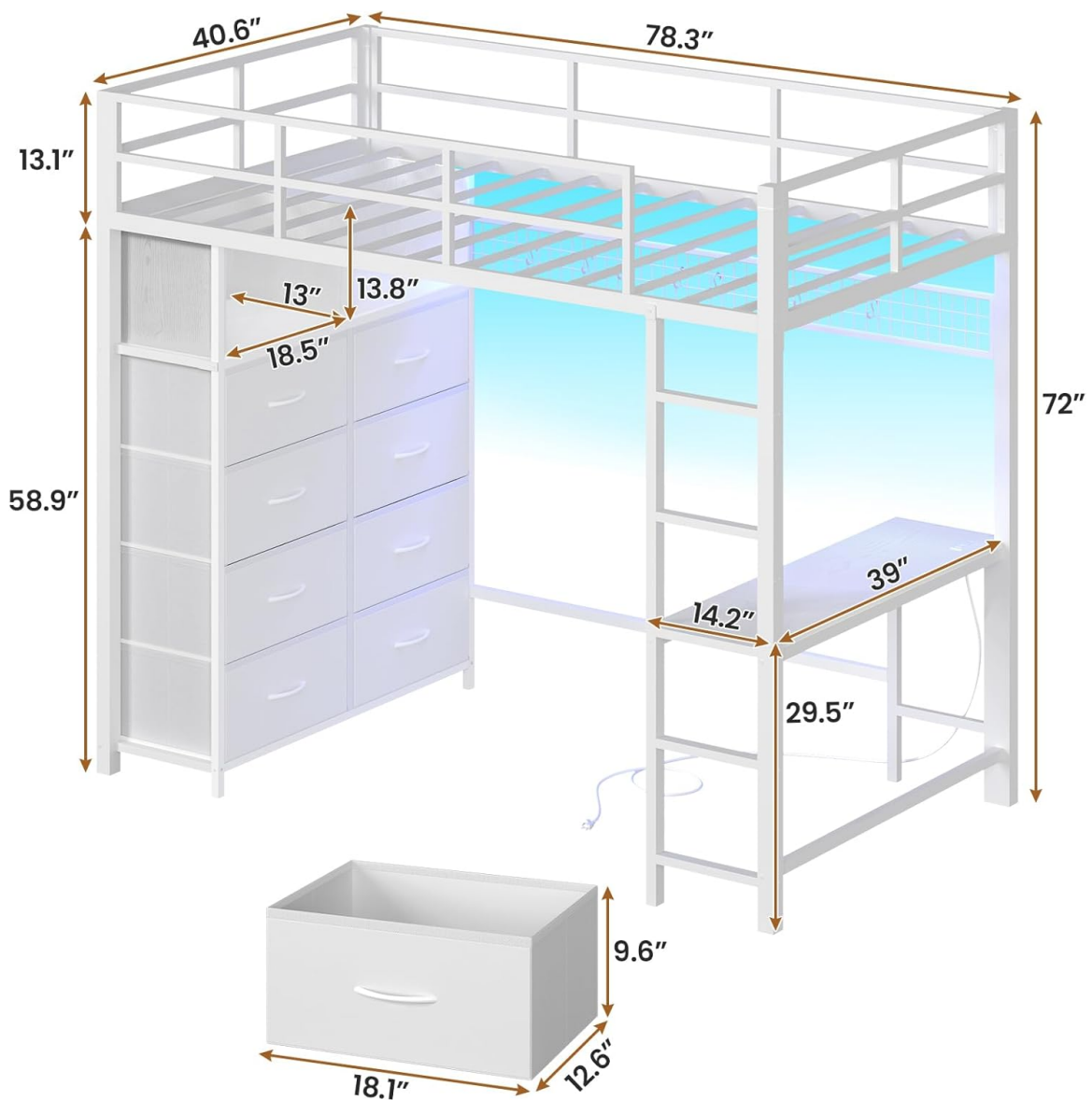
A diagram showing the key dimensions of the loft bed, including height, length, and width.
