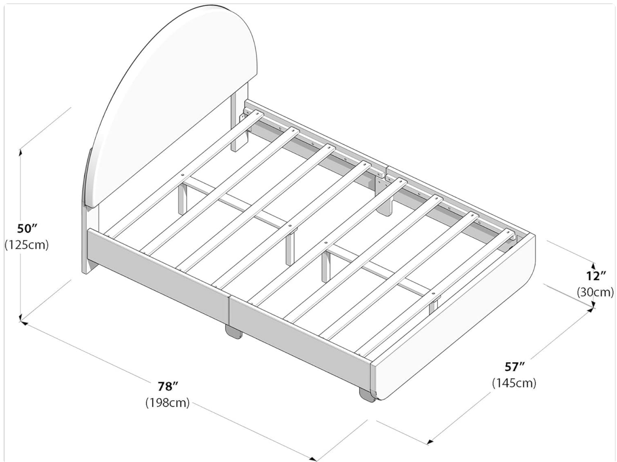
Figure 2.1: Bed Frame Dimensions (78.75" L x 58.5" W x 50.5" H)
