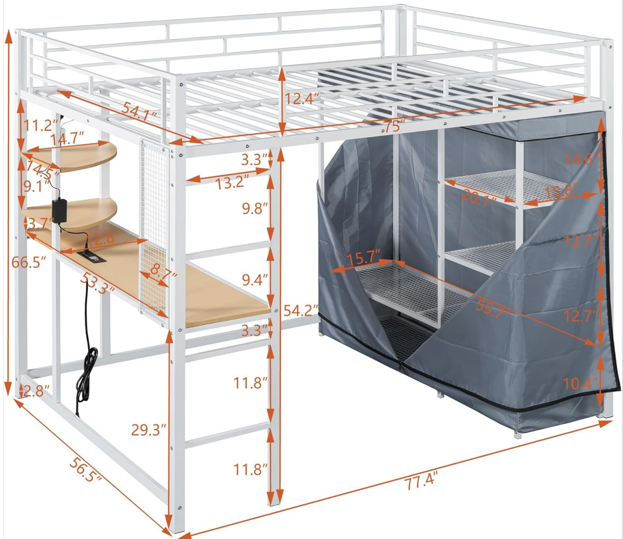
Image: Detailed diagram showing the dimensions of the Merax Full Size Metal Loft Bed in inches, including length, width, and height of various components like the bed frame, desk, and wardrobe area.
