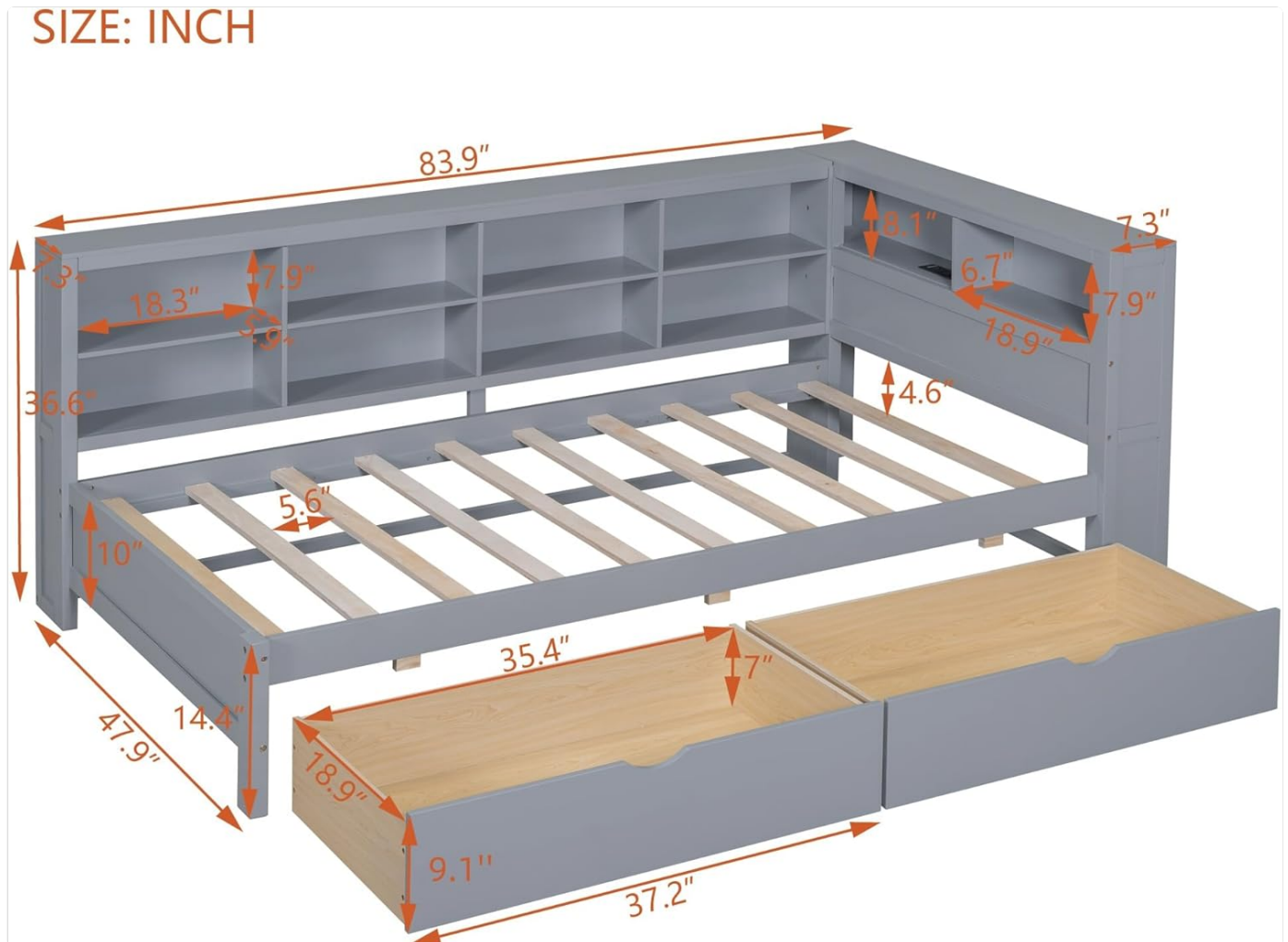
Image 6: Dimensional diagram of the daybed, illustrating length, width, height, and internal measurements of shelves and drawers.
