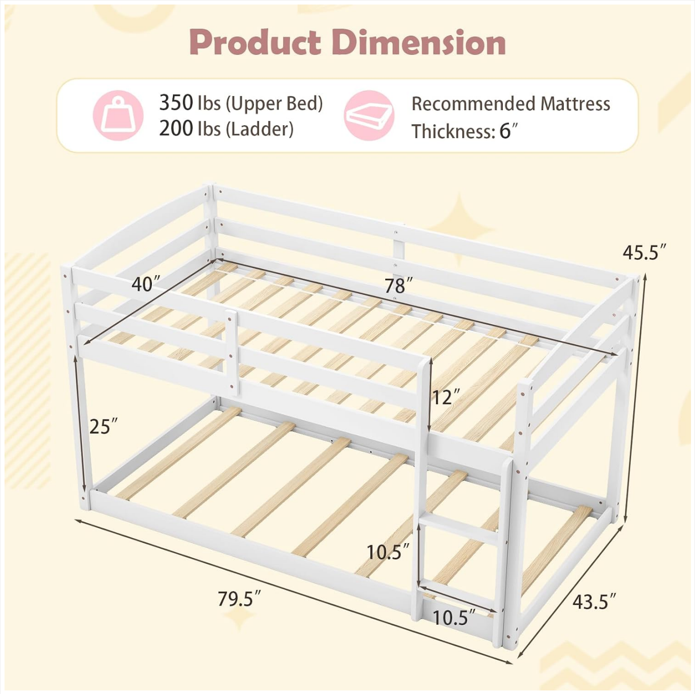
Image: Detailed product dimensions and weight capacities for the IFANNY Low Bunk Bed.
