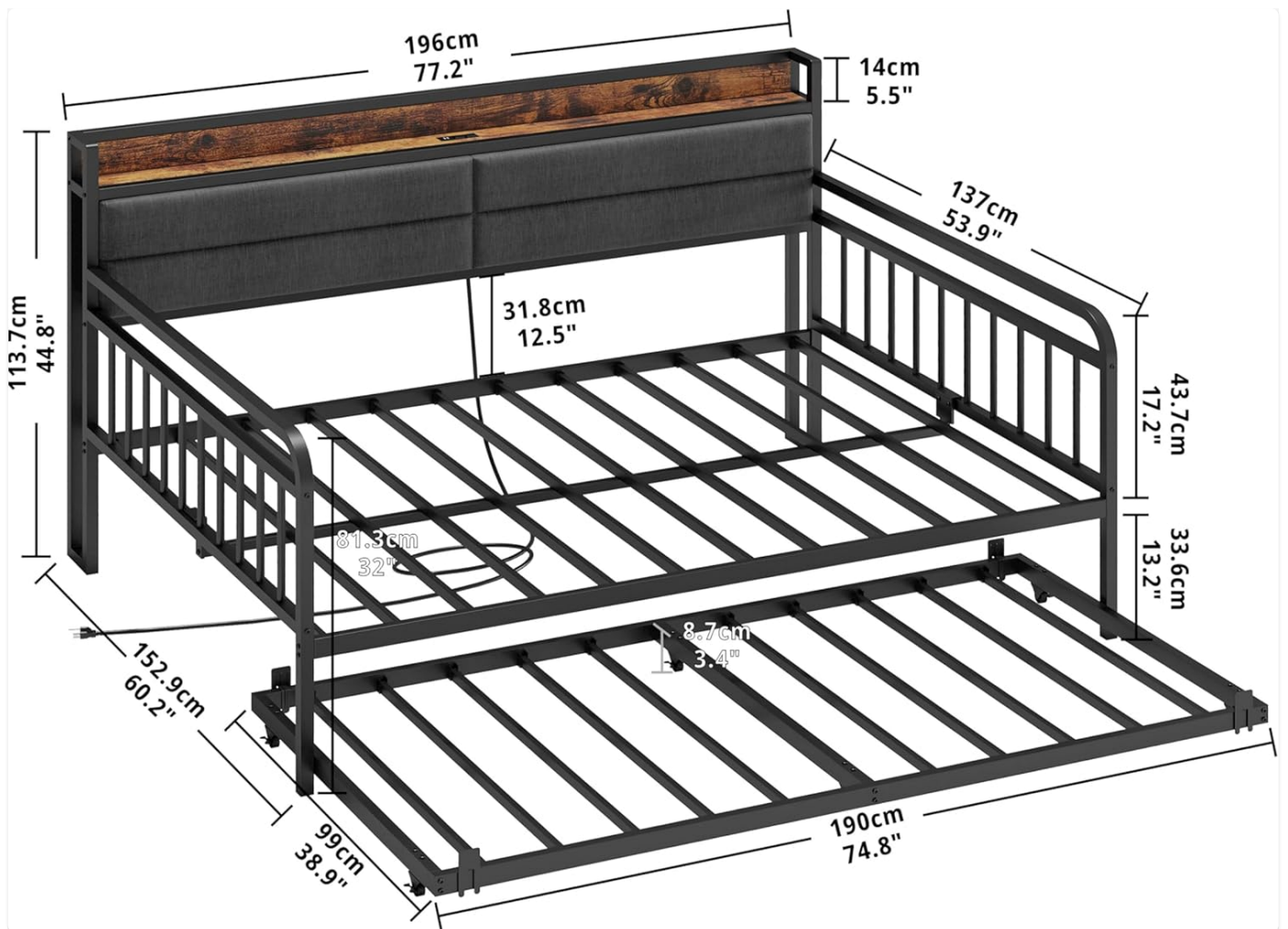
Image: Detailed dimensions of the LIKIMIO Daybed with Trundle, showing measurements in both centimeters and inches.
