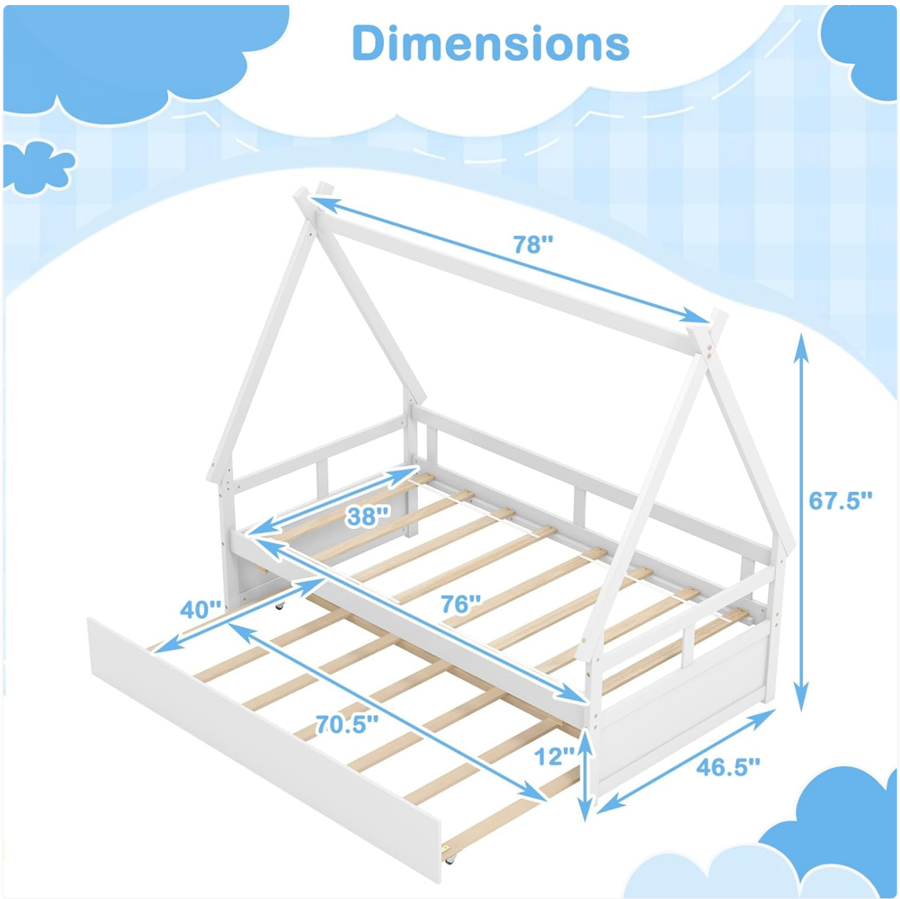
Image 8.1: Detailed dimensions of the bed and trundle components.
