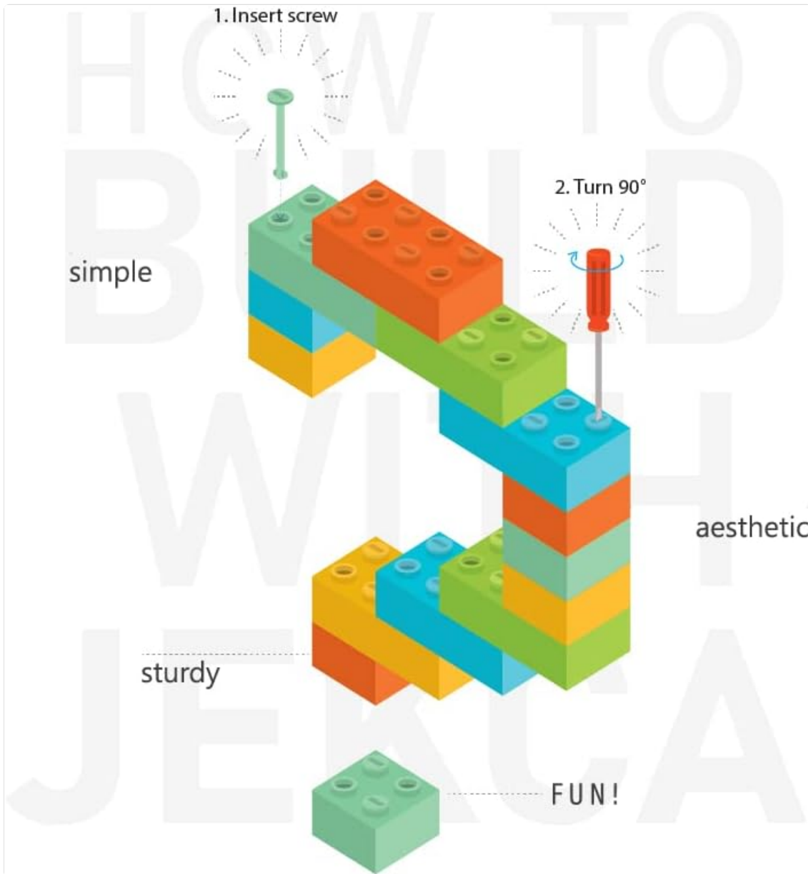
Figure 2: Illustration of the JEKCA interlocking system. Insert the pin (screw) and turn 90 degrees with the pin driver to secure the bricks.
